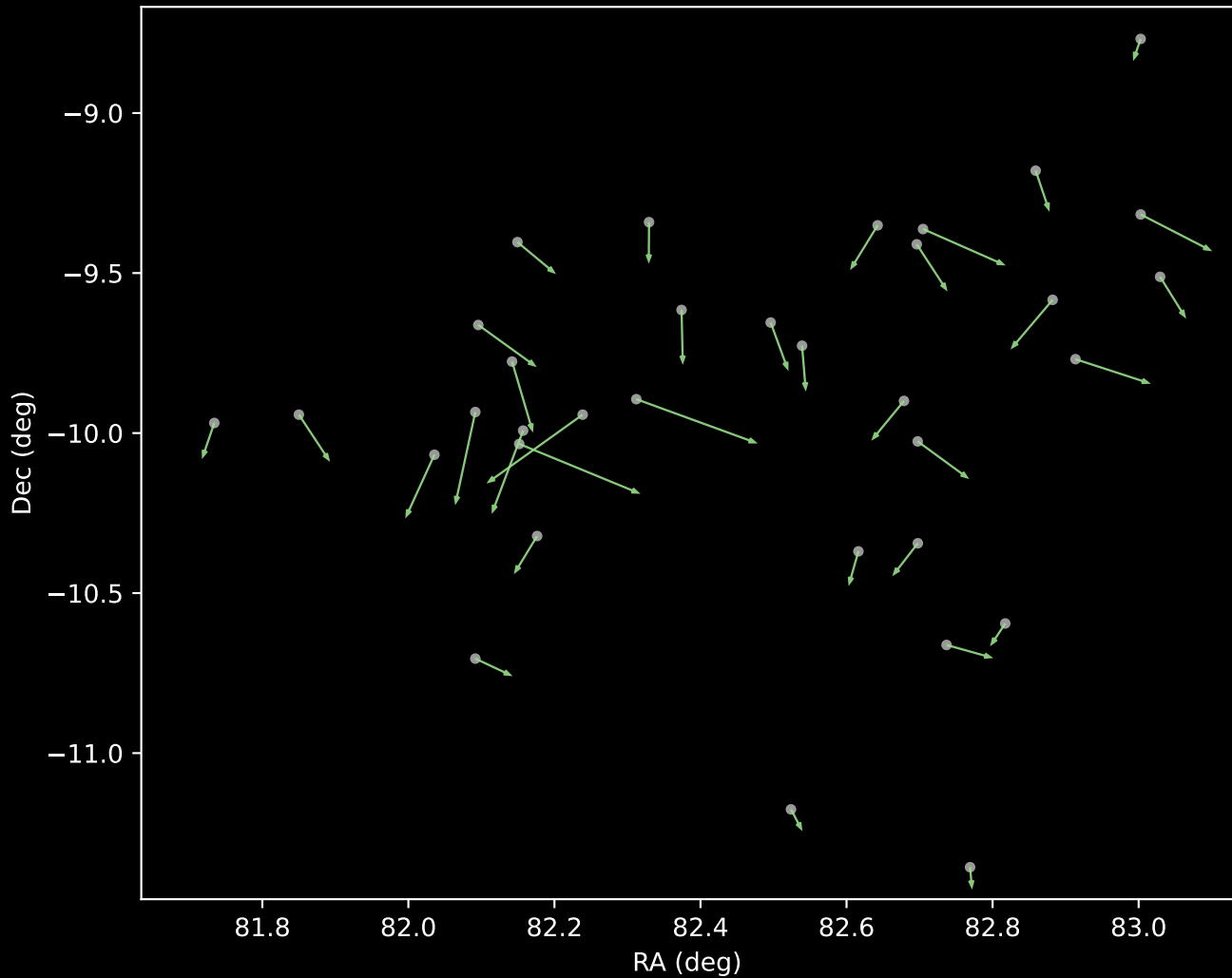
APOGEE DR17 Cluster 5 Proper Motion Vectors (n=34)
