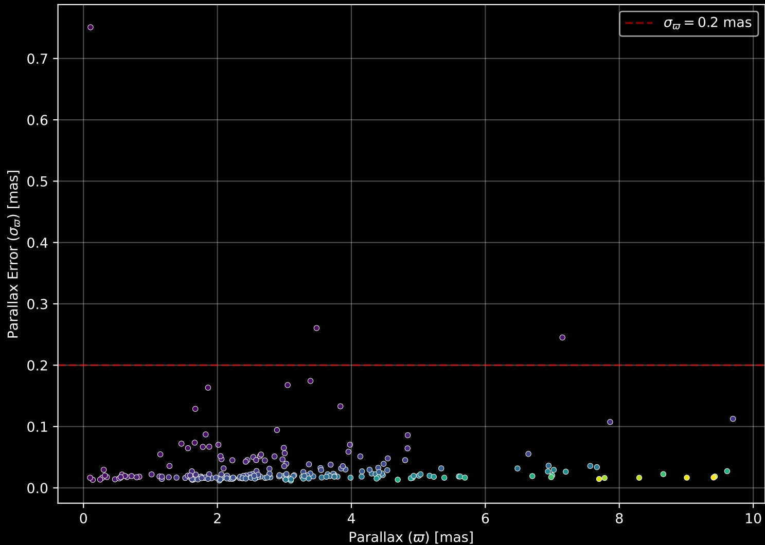
APOGEE DR17 Field: [K2_C3_059-57] Parallax Quality (n= 216)
