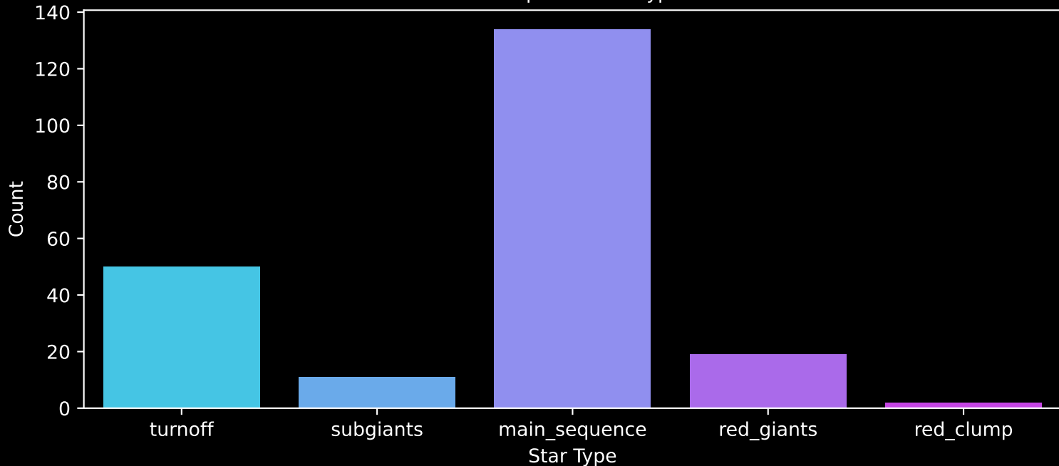
APOGEE DR17 Field: [K2_C3_059-57] Count plot of Star Type
