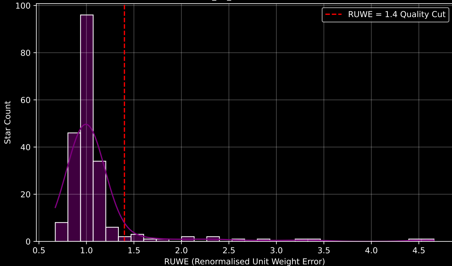
GAPOGEE DR17 Field [K2_C3_059-57] RUWE Distribution (n= 207)
