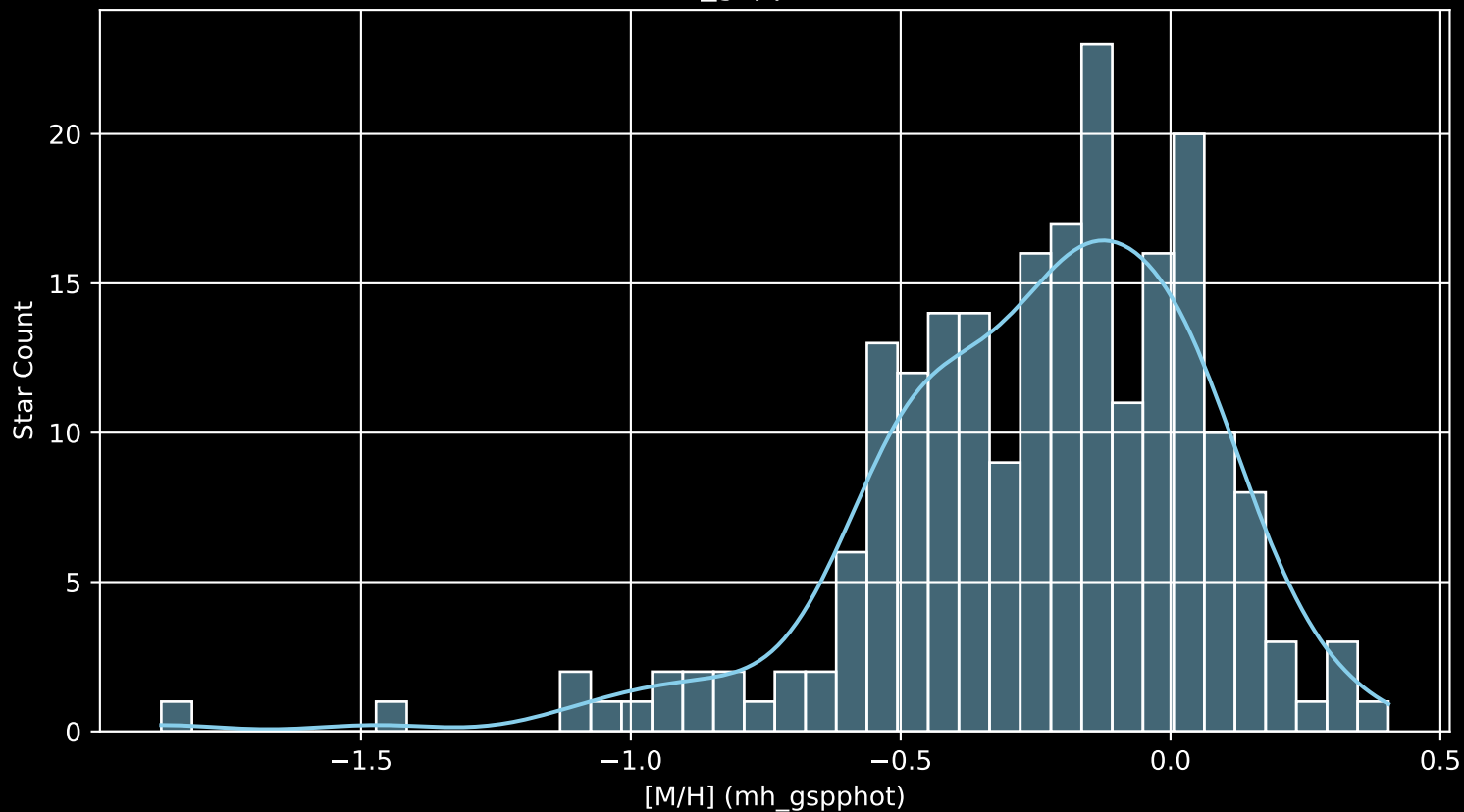
APOGEE DR17 Field: [K2_C3_059-57 [M/H] (mh_gspphot) (n= 214)
