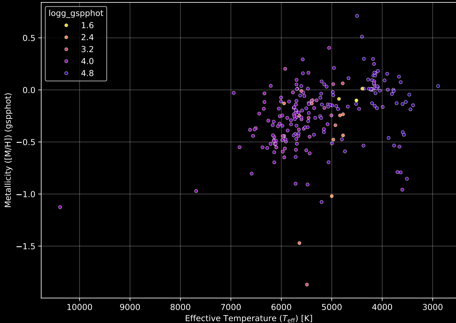
APOGEE DR17 Field: [K2_C3_059-57] Stellar Population Parameters (n= 216)
