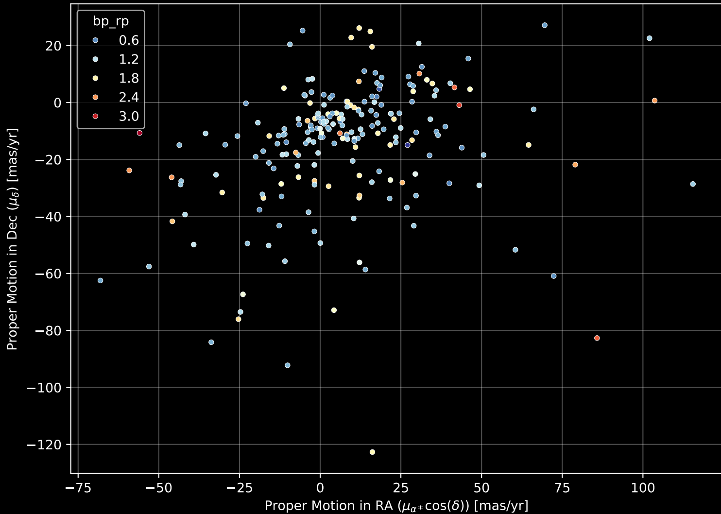
APOGEE DR17 Field: [K2_C3_059-57] Proper Motion Diagram (n= 216)
